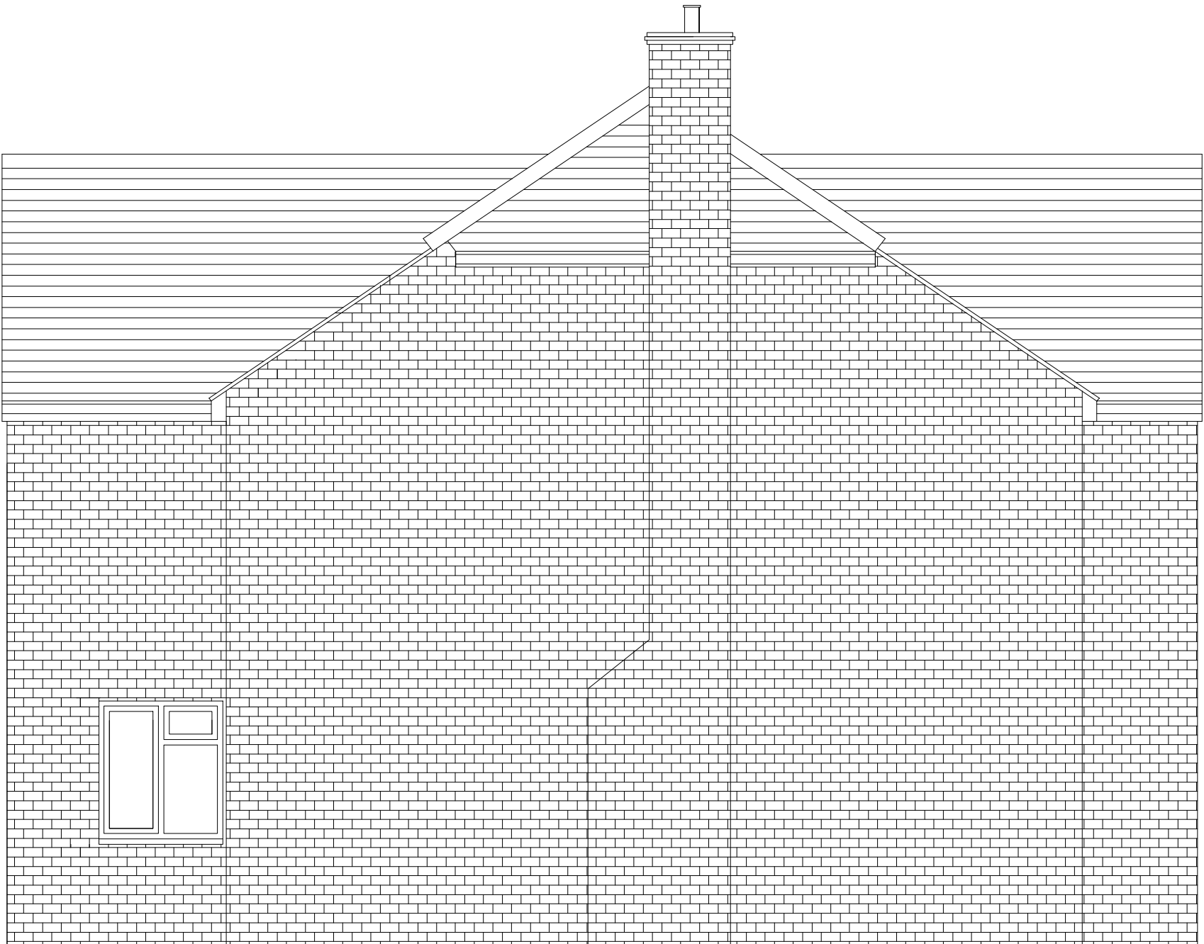
EXISTING ELEVATION B SIDE
